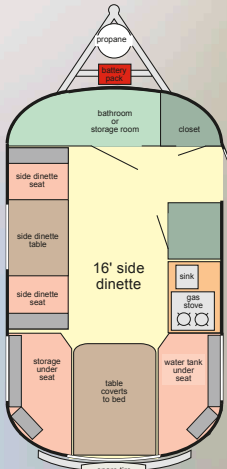
Layout 6
