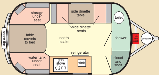
Layout B Side Dinette
