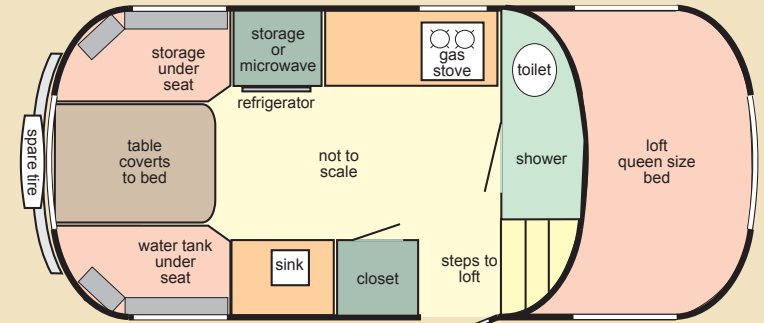
Layout B
