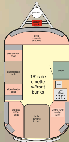
Layout 7
