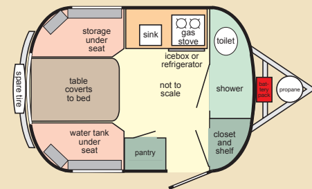
Layout B With Shower and Toilet
