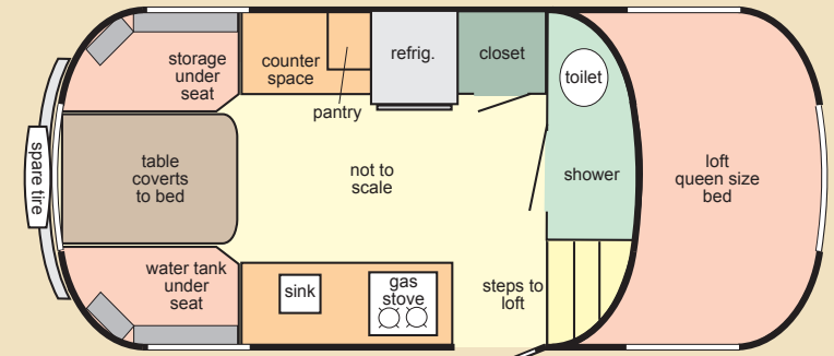
Layout A
