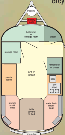
Layout 5
