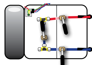
Shown in Bypass Configuration (levers vertical)
